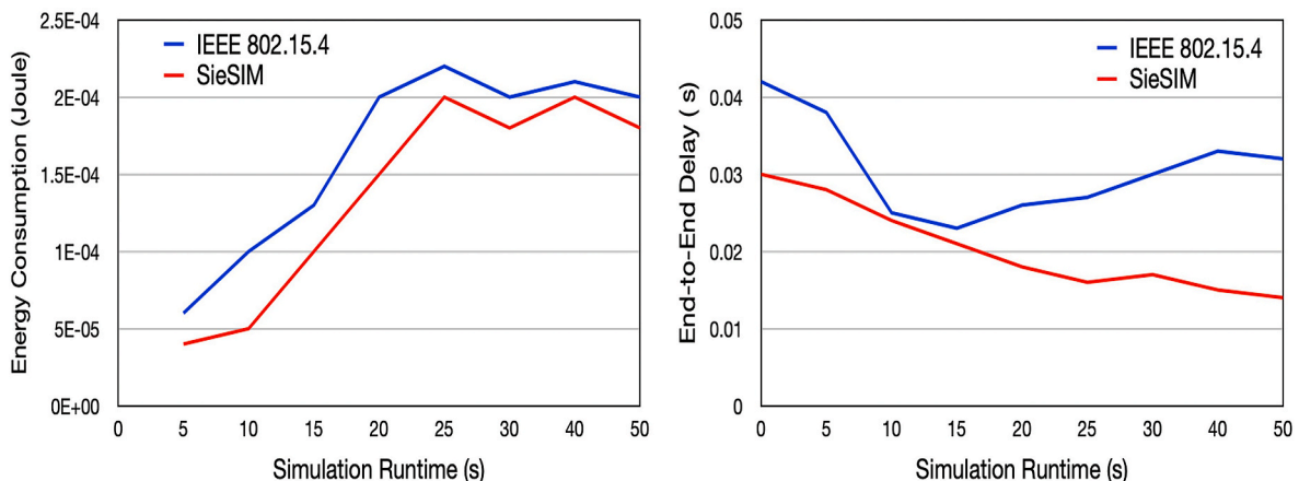
Fig. 16. a) Energy Consumption b) End-to-End delay.
