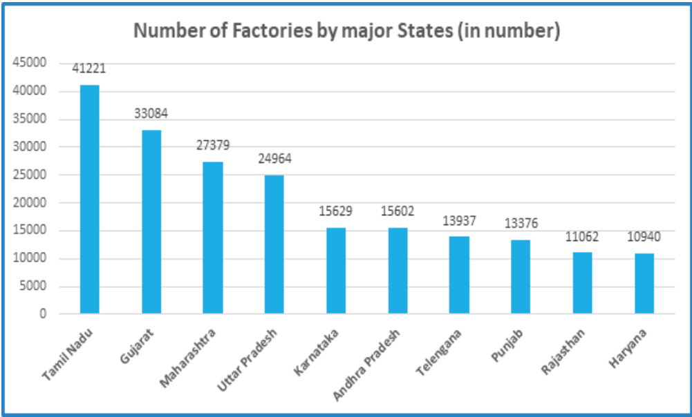
Chart-1: Bar chart showing the Number of factories by major States in ASI 2024-25: All India
