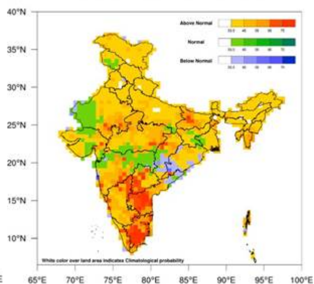
Fig.4b. Probability forecast of Minimum Temperature for June 2026.
