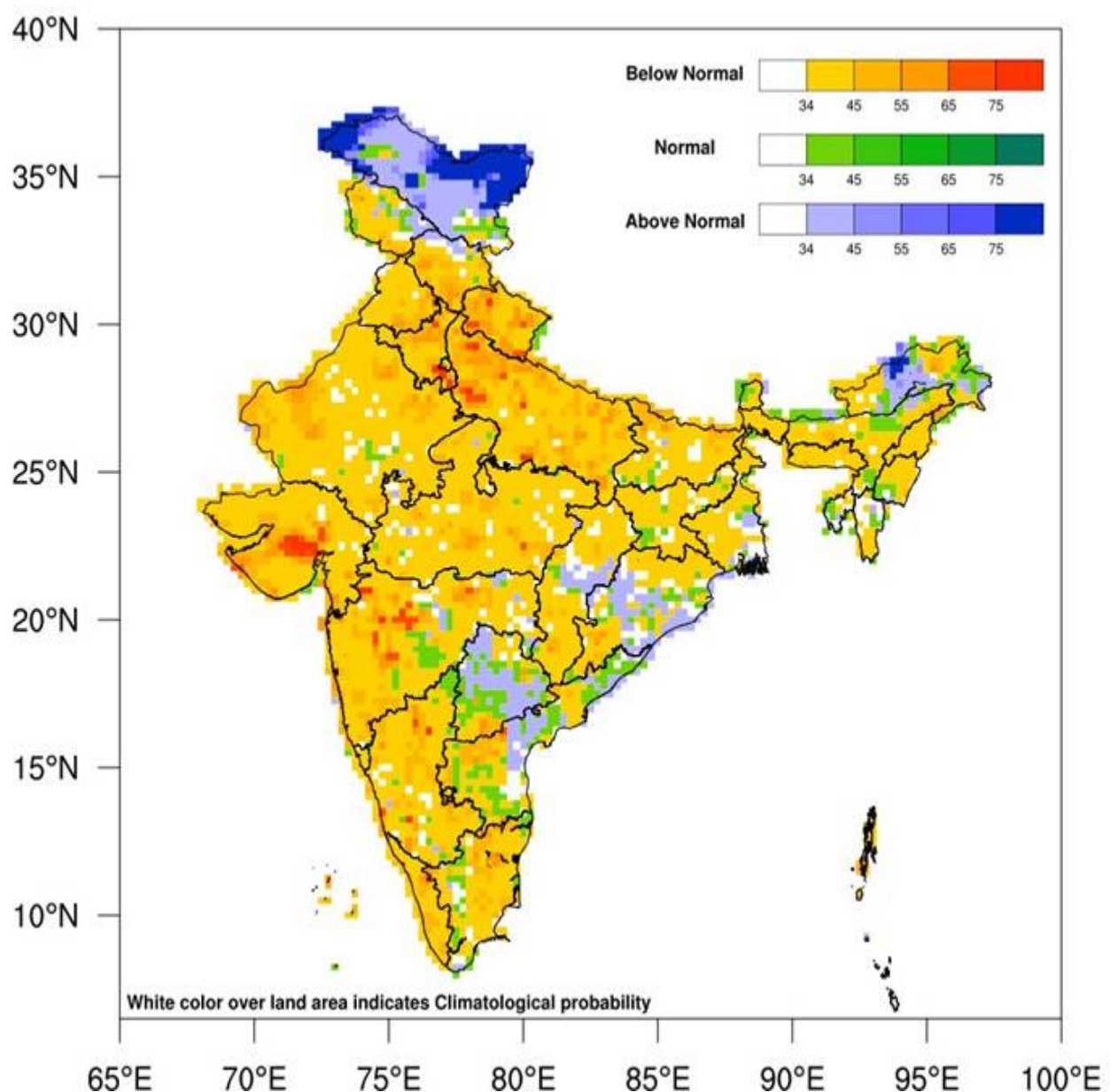
Fig.1. Updated Probability forecast of tercile categories* (below normal, normal, and above normal) of rainfall over India during southwest monsoon season (June-September), 2026. The figure illustrates the most likely categories as well as their
