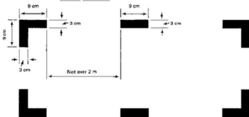
Figure 2.4-1 MARKING OF BREAK-IN POINTS (see 2.4.2.6)
