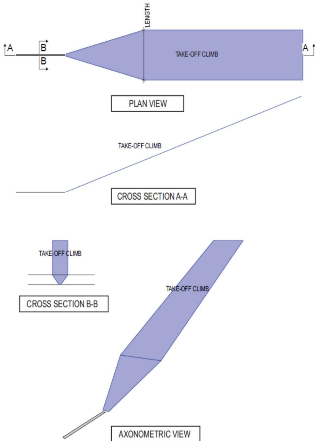
Figure 4-8 Take-off climb surface
