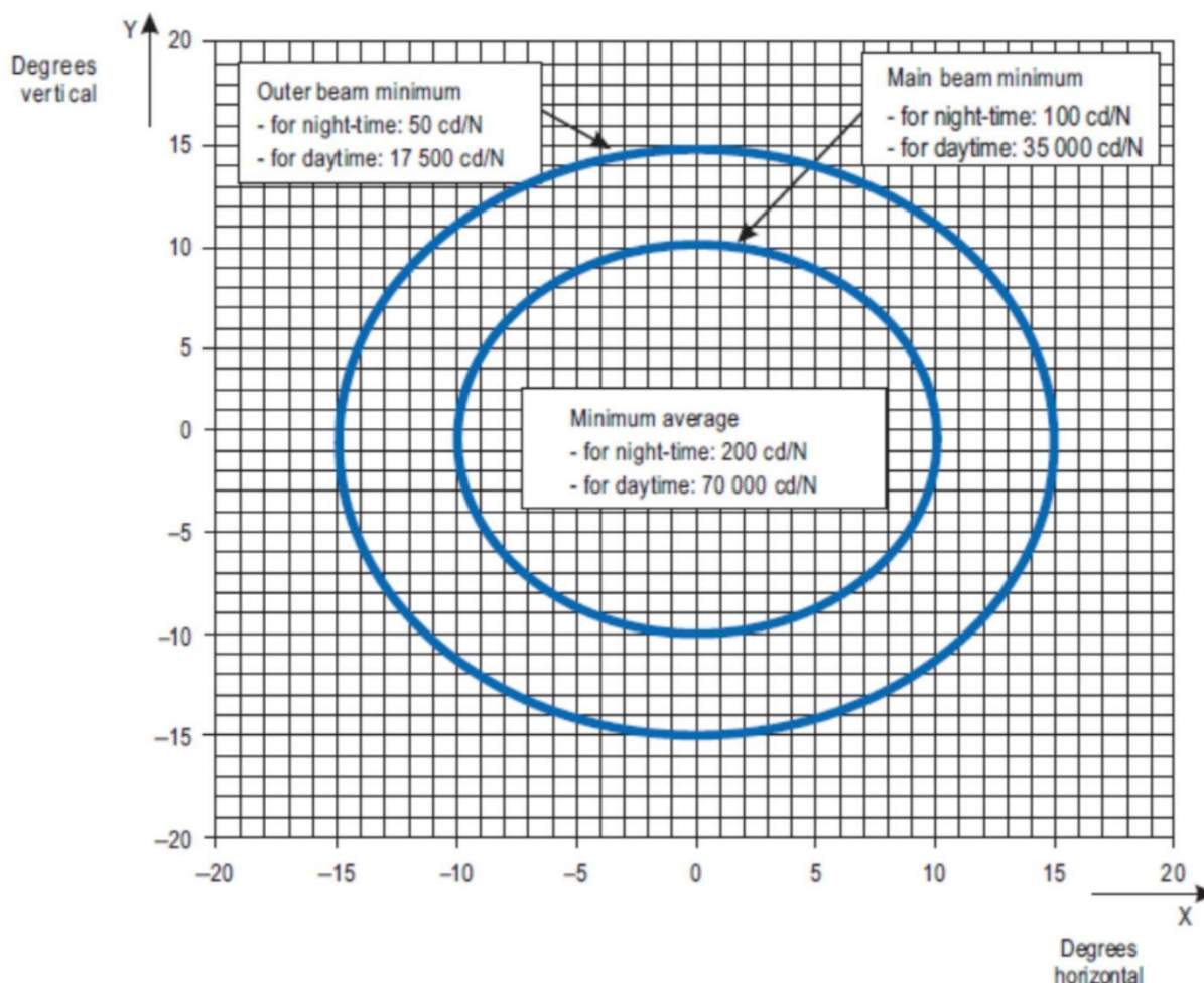
Figure A2-26. Isocandela diagram for take-off and hold lights (THL) (red light)
