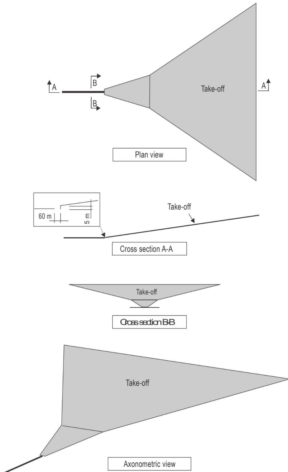
Figure 4-7. Instrument departure surface
