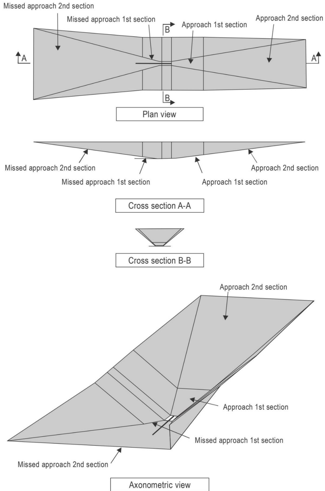
Figure 4-6. Surface for precision approaches
