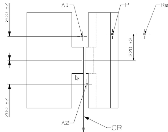
"Re" is located on the centre line of the retractor spool
