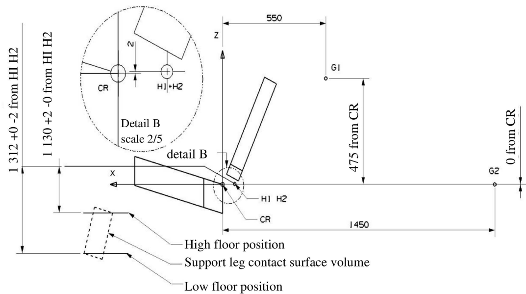
Side View – Bench with anchorages (Dimensions in mm; Tolerance general: ±2 mm)
