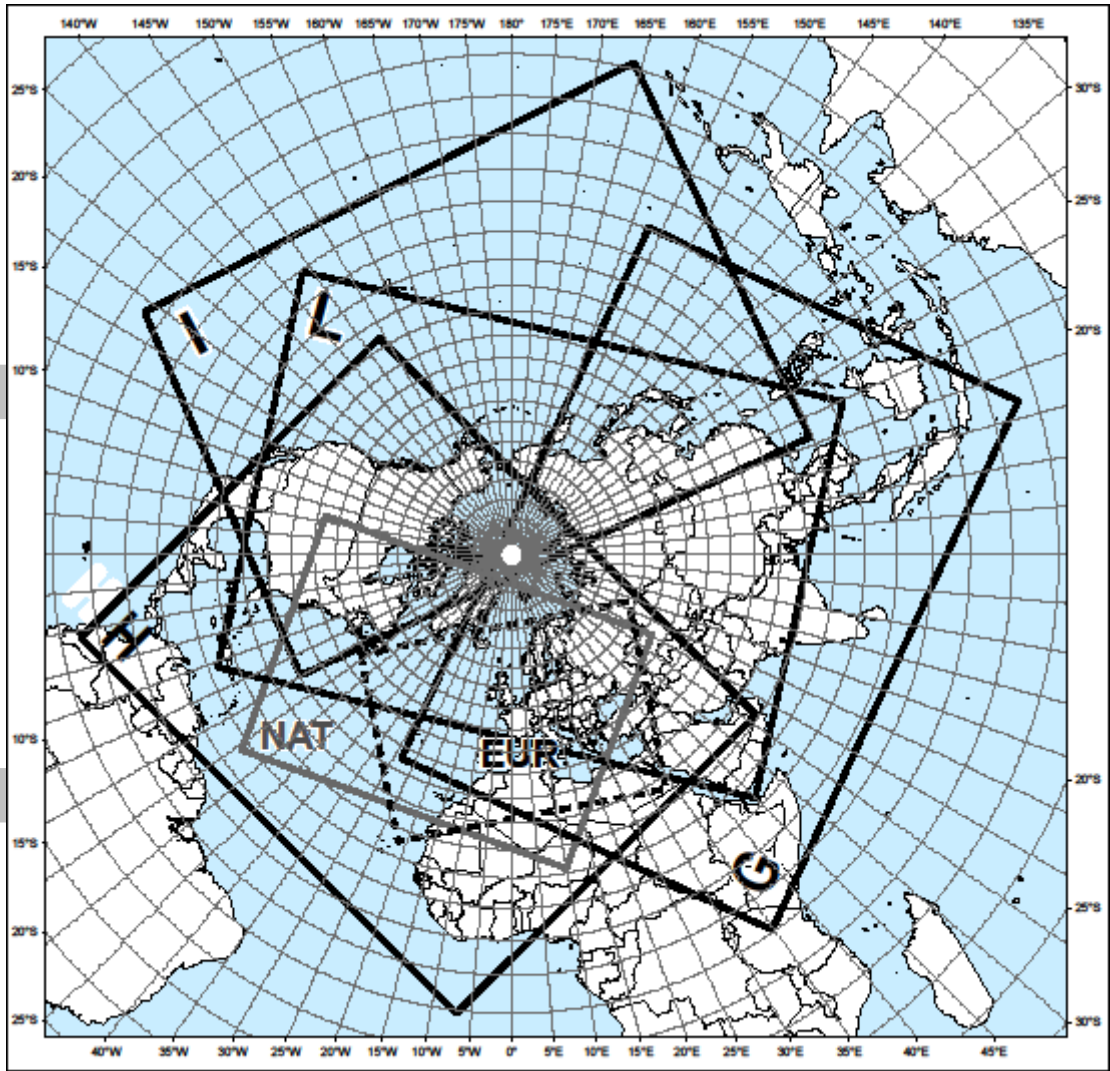
Figure A8-1: Fixed areas of coverage of WAFS forecasts in chart form — Mercator projection
