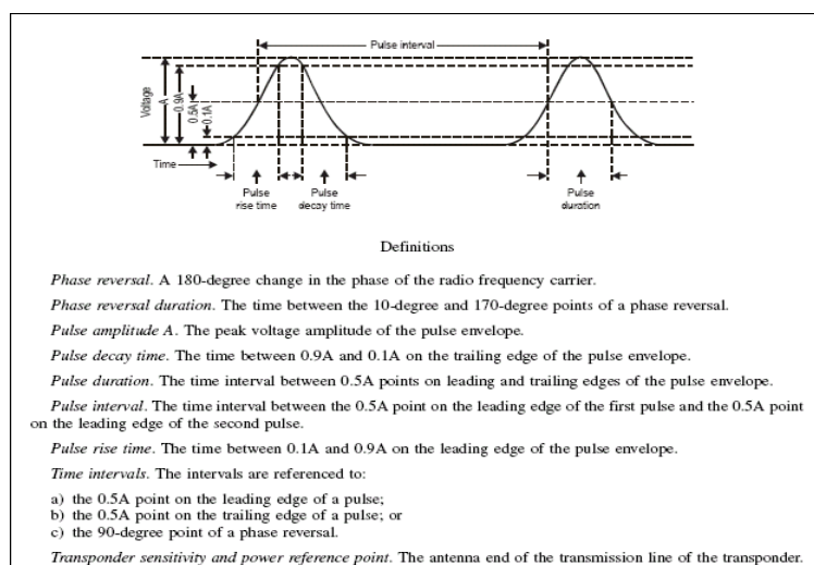
Figure 3-1. Definitions of secondary surveillance radar waveform shapes, intervals and the reference point for sensitivity and power.
