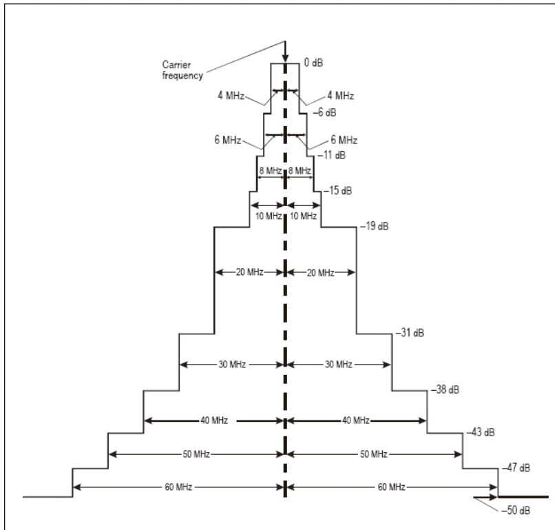
Figure 3-2. Required spectrum limits for interrogator transmitter
