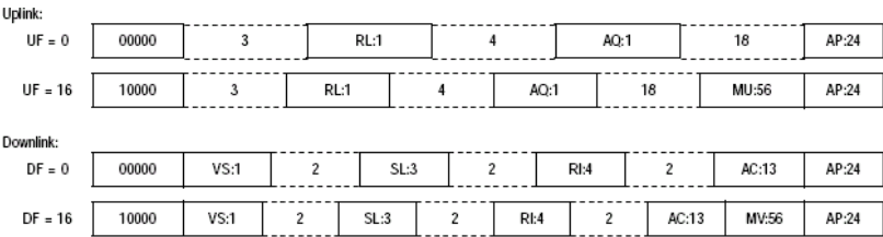
Figure 4-1. Surveillance and communication formats used by ACAS
