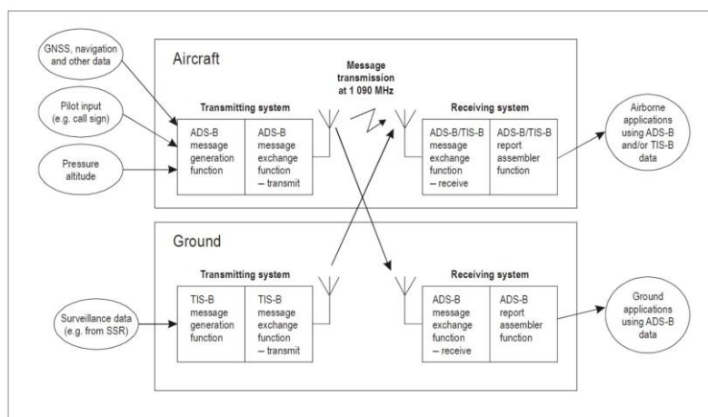
Figure 5-1. ADS-B/TIS-B system functional model
