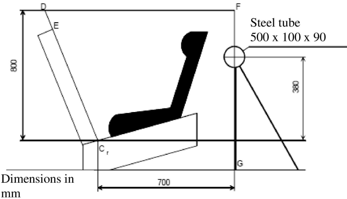
Arrangement for testing a rearward-facing device, not supported by the dashboard
