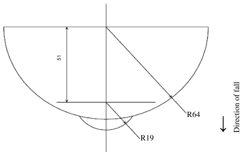
Headform
