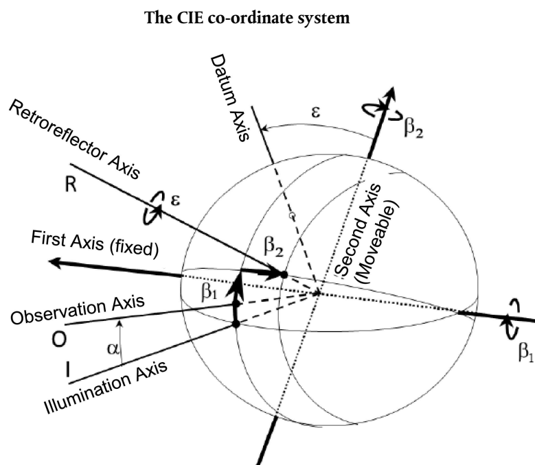
Figure A4-I shows the CIE angular system for specifying and measuring retro-reflective device and marking materials. The first axis is perpendicular to the plane containing the observation axis and the illumination axis. The second axis is perpendicular both to the first axis and to the reference axis.
