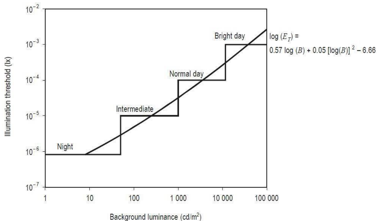
Figure D-1. Relationship between the illumination threshold E_T(\text{lx}) and background luminance B(\text{cd/m}^2)
