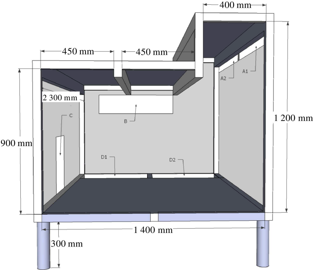
Framework for the test apparatus
