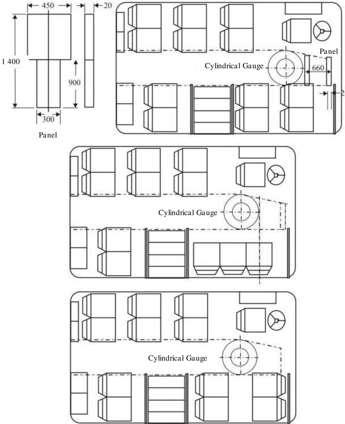
Figure 7 Forward limitation of the gangway (dimensions in mm) (See Annex 3, paragraph 7.7.5.1.1.1.)
