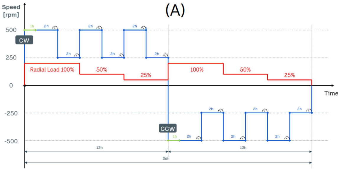
Testing sequence scheme A
