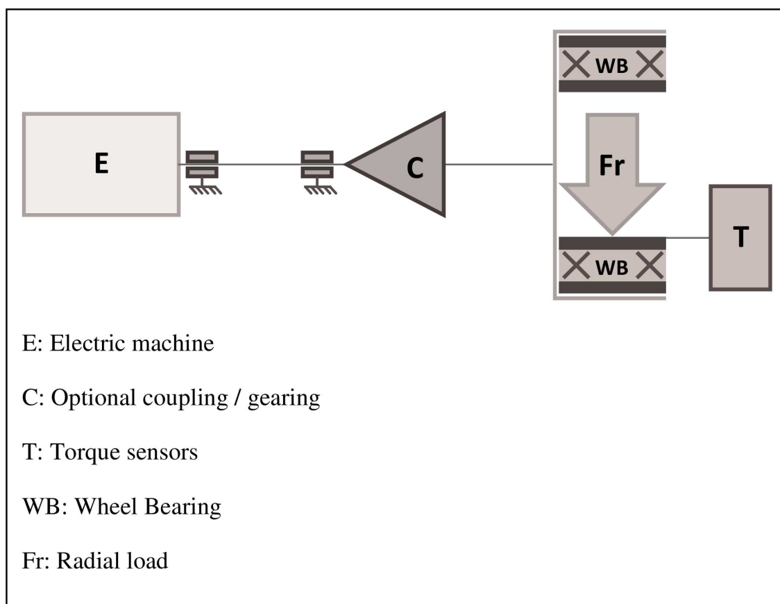
Simplified schematic of the test set-up
