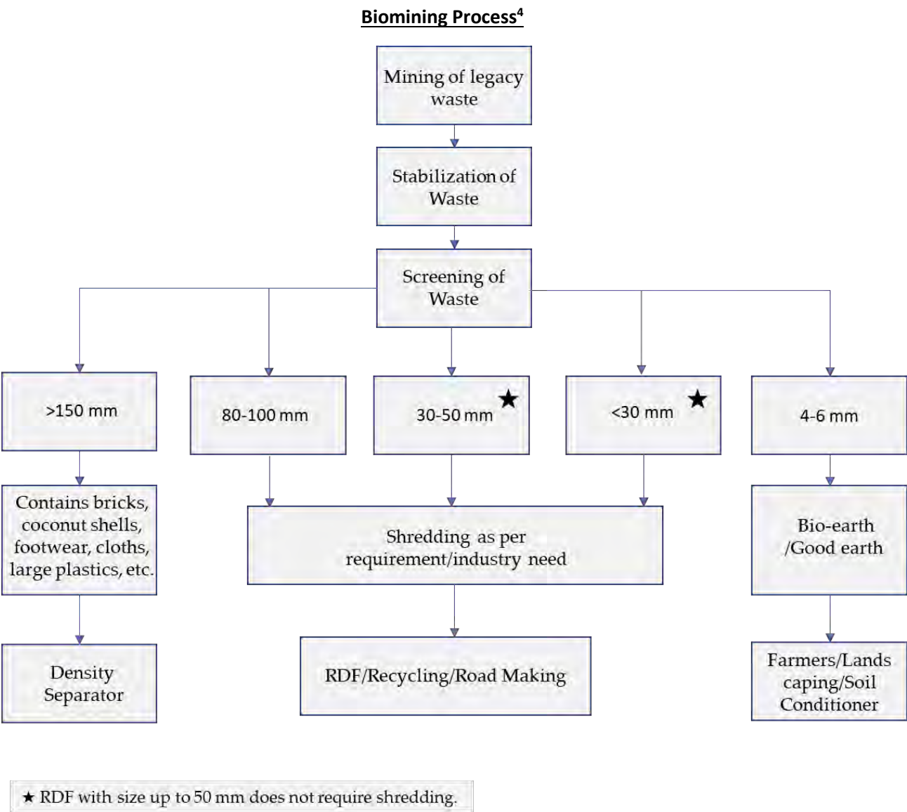
Figure 4: Biomining Process
